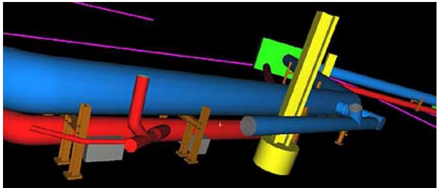
High Definition Survey – Prudential Center Complex
